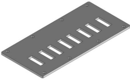
KTL-H-8-30
